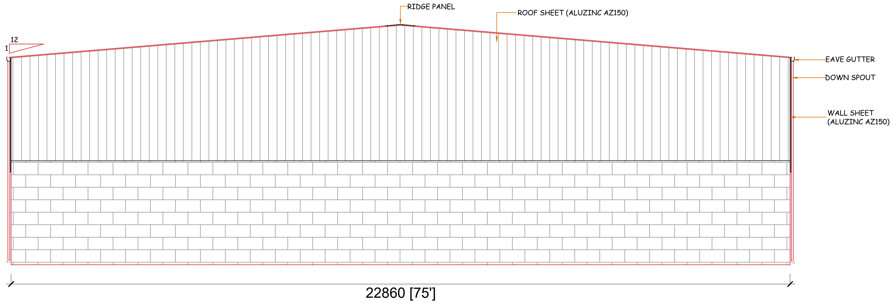
REAR ELEVATION
