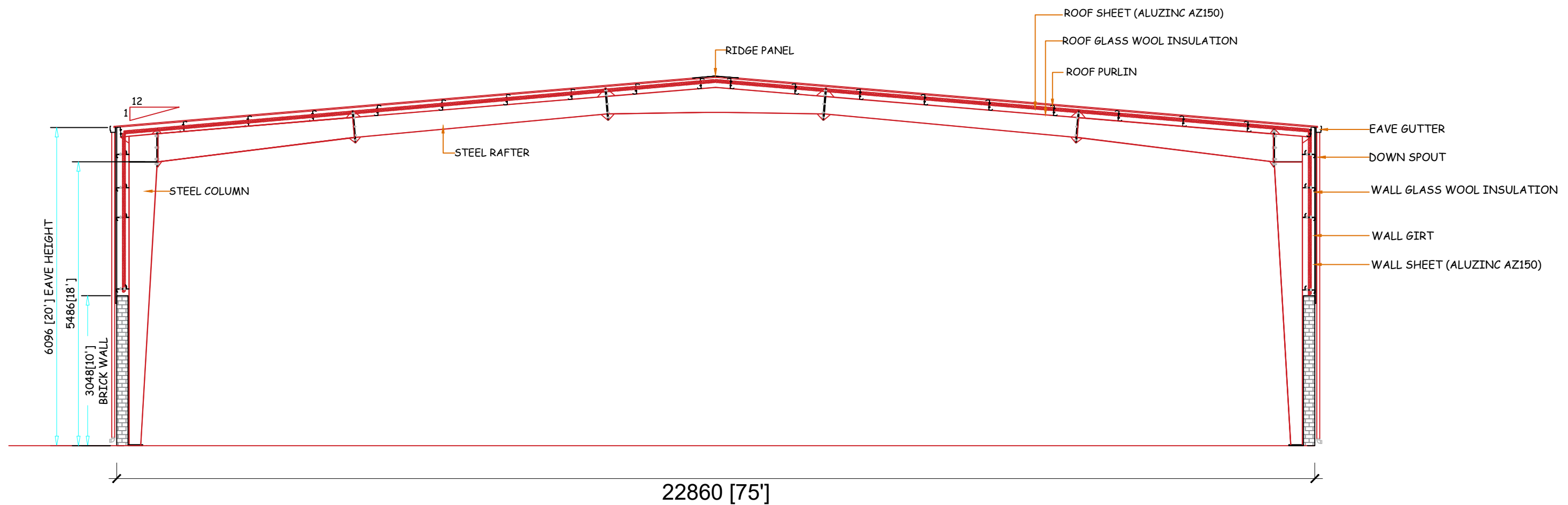
MAIN FRAME SECTION
