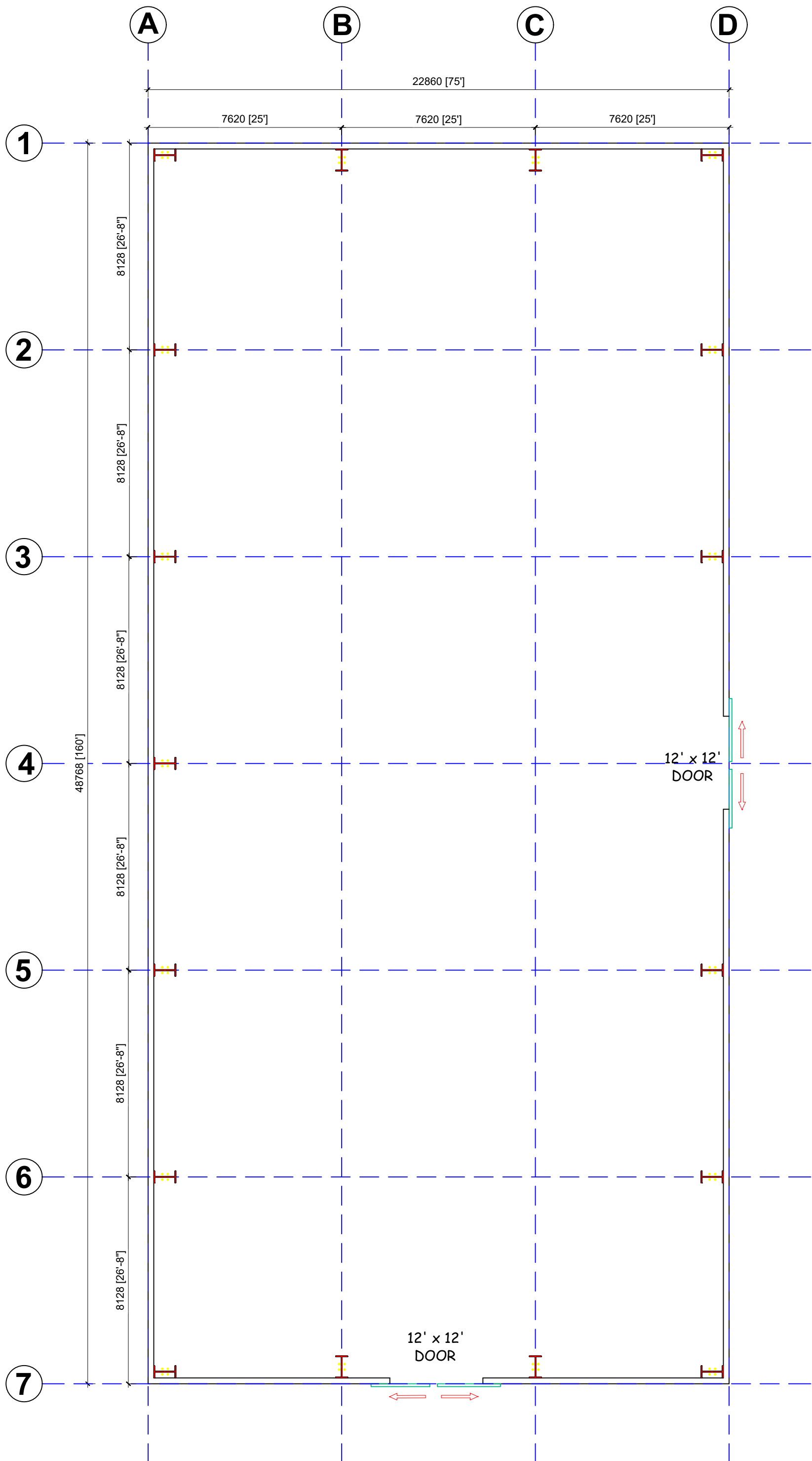
LAYOUT PLAN
