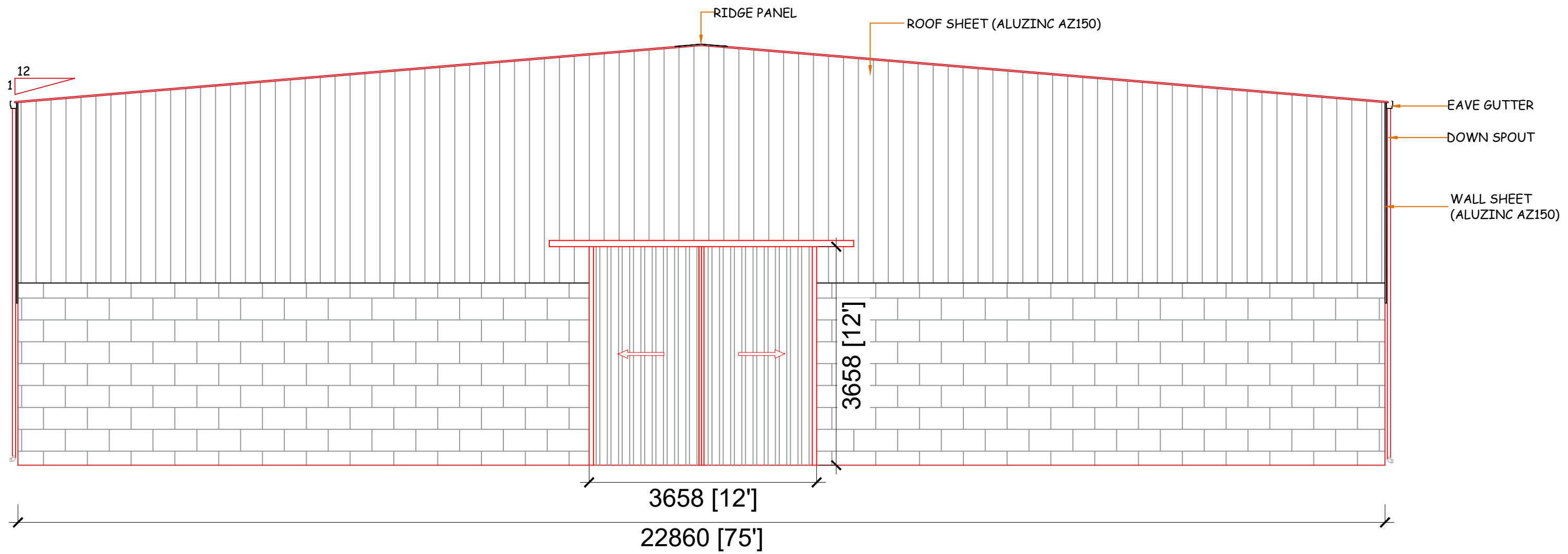
FRONT ELEVATION
