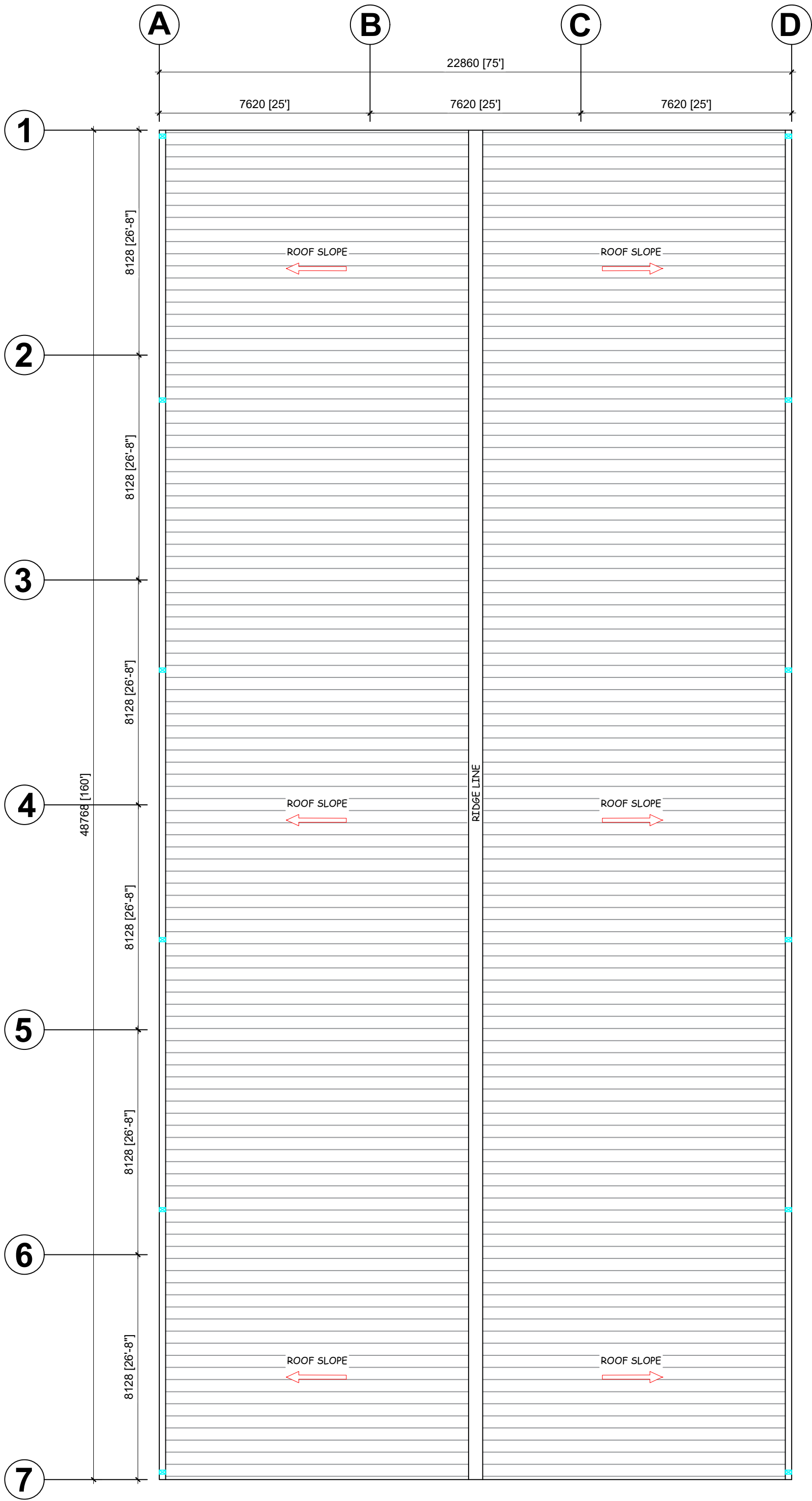
ROOF PLAN
